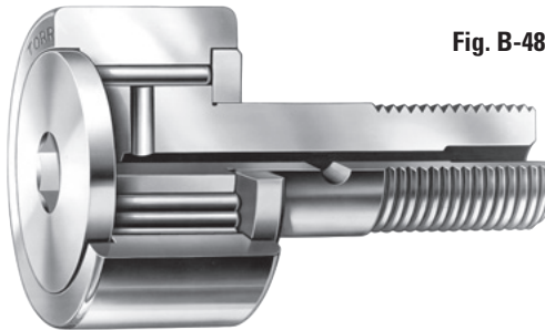
Fig. B-47. Stud-type track rollers
