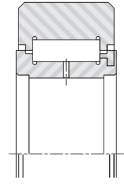
FGU/FGUL Heavy
