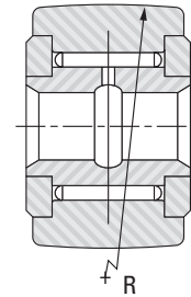
Fig. B-64. YCR for yoke mounting
