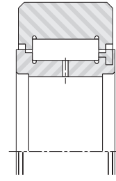
FGU/FGUL Light
