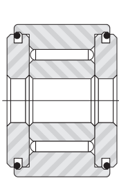
FP/FPL
